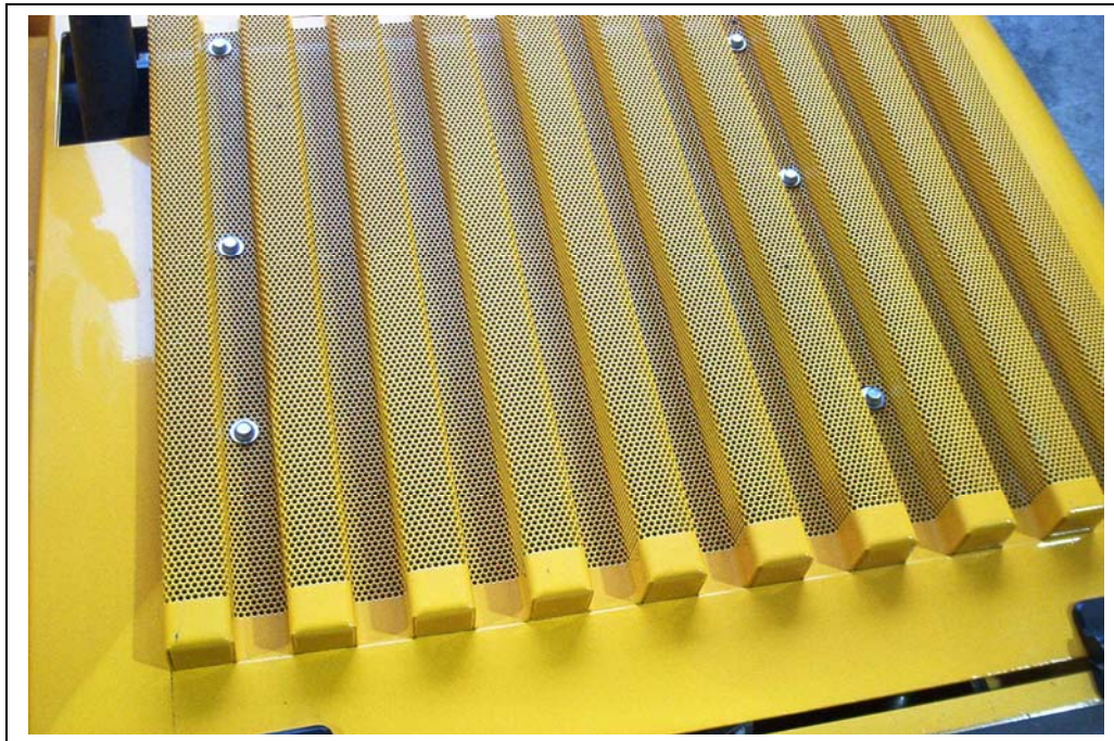
Top of engine lid with bolt heads visible and the condenser under the lid.
