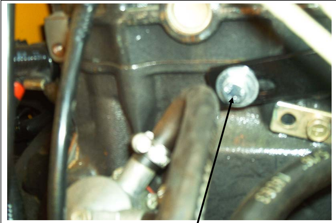
Compressor stiffener bracket bolts to the engine block.
