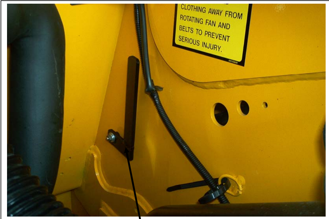
Drier bracket installed with 1/4" hardware provided.
