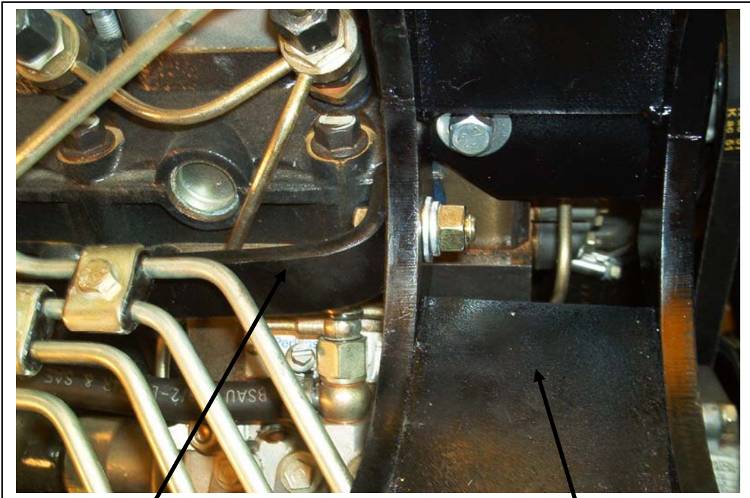
Stiffener bracket
